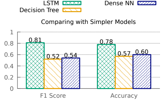
Fig. 2. The F_1 score and accuracies of the different ML models train on the Laghos data set. Only the LSTM achieves reasonable results, which emphasizes the necessity of preserving the entire edit script.
